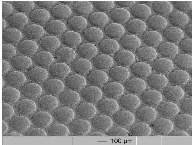
Figure 1: lens array
