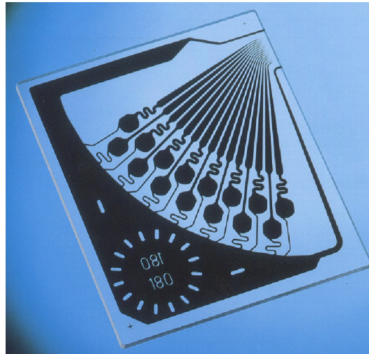
Figure 1 : Mikroglas component for inkjet printhead : nozzles, channels, chambers
